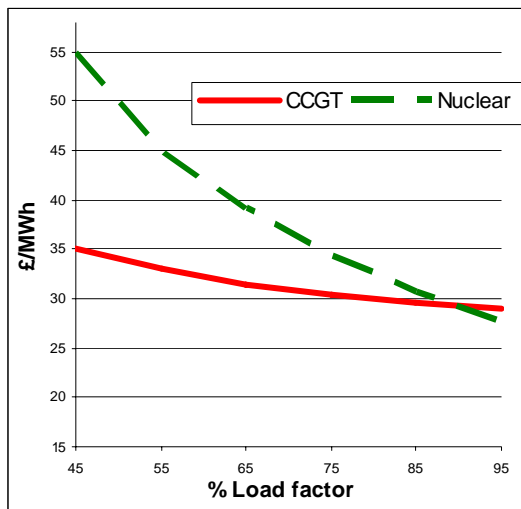
Figure 4.2 – sensitivity of levelised costs to plant load factor variation
