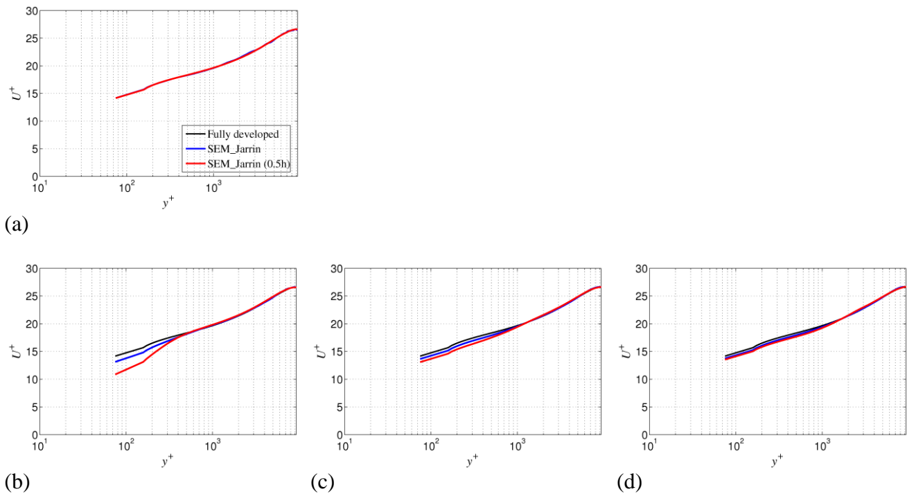
Figure 3.21: development of mean-velocity with synthetic turbulence (SEM_Jarrin); \text{Re}_\tau = 9300 ; (a) x/h = 0 ; (b) x/h = 2 ; (c) x/h = 4 ; (d) x/h = 6 .
