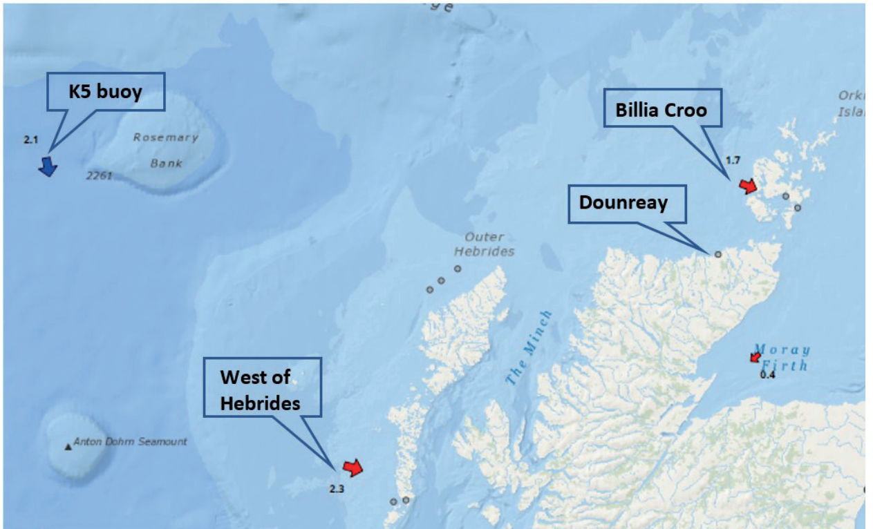
Figure 9. WaveNet map showing the location of current deployments (red and blue arrows) and historical deployments (grey circles) around Downreay. Significant wave height is reported in metres (numbers on the map), as measured by buoys on 27/04/2018 at 14:00hrs; date and time are almost real time on the live online map, wave direction is indicated by red arrows and wind direction by blue arrows. (Source: Cefas (2018); © Crown Copyright 2018)
