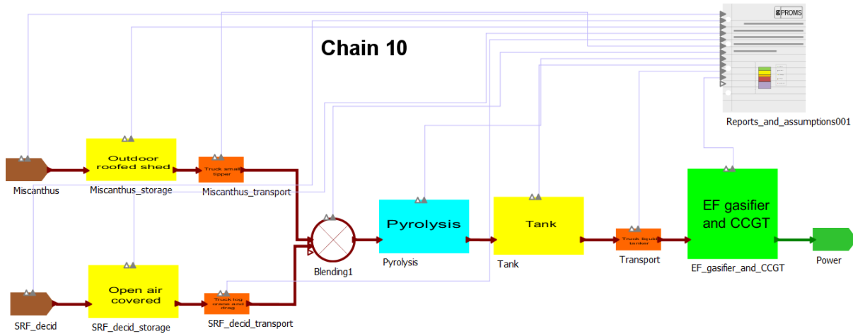
Figure 4.19: Chain 10 architecture in gPROMS
