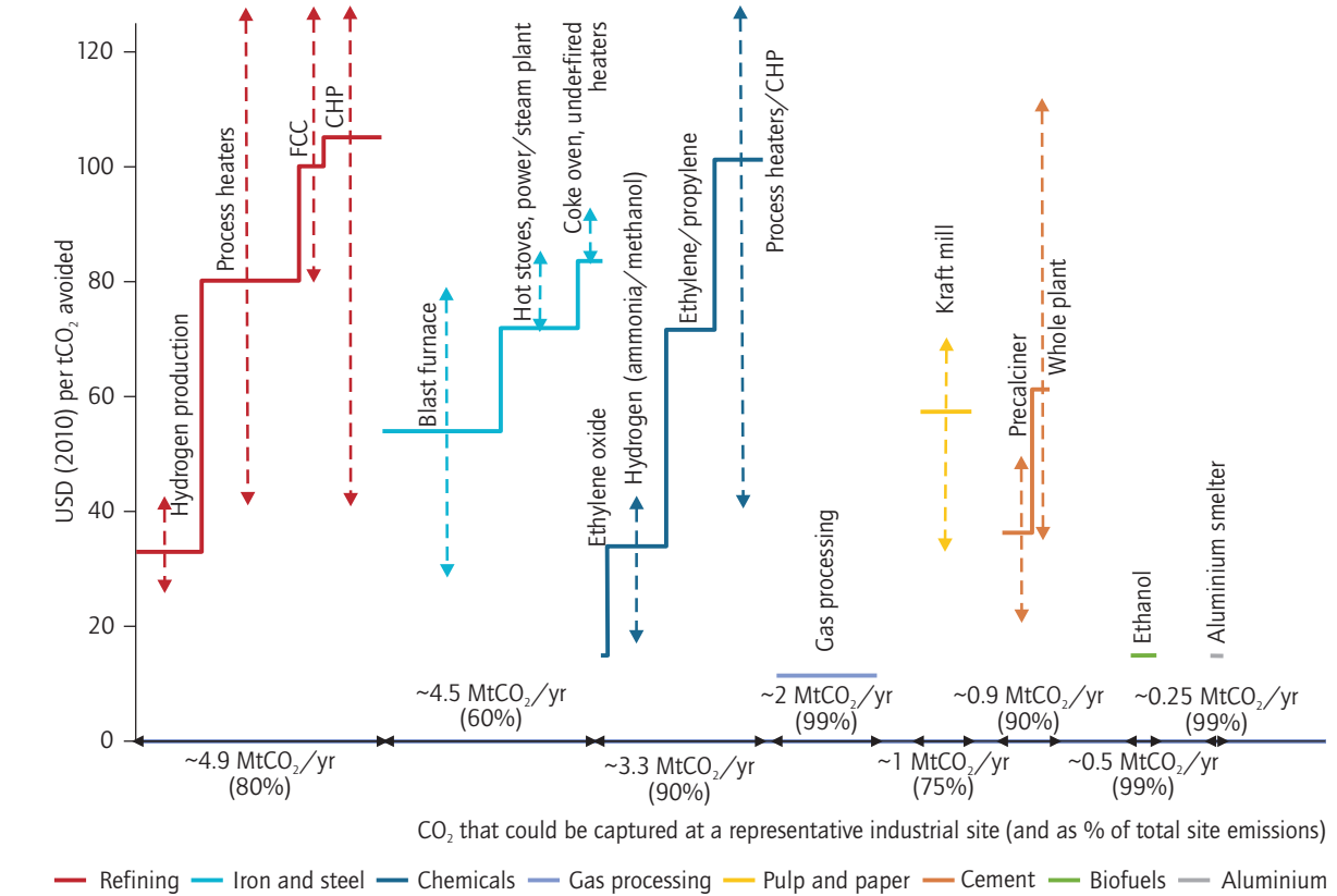
Figure 11: Illustration of CO 2 avoidance costs and sizes of CO 2 sources for capture at archetypal industrial sites
