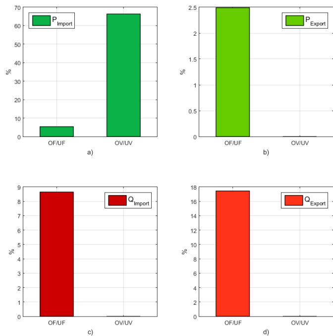
Figure 33. OF,UF,OV,UV NDZs for Generation Mix 4, a) Active power import, b) Active power export, c) Reactive power import, d) reactive power export
