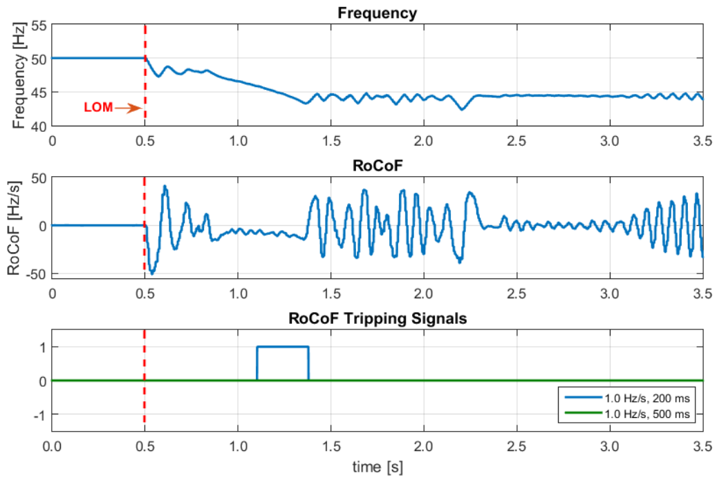
Figure 8. Islanded system response for generation mix 7 (75% PV + 25% DFIG) – 15% reactive power export
