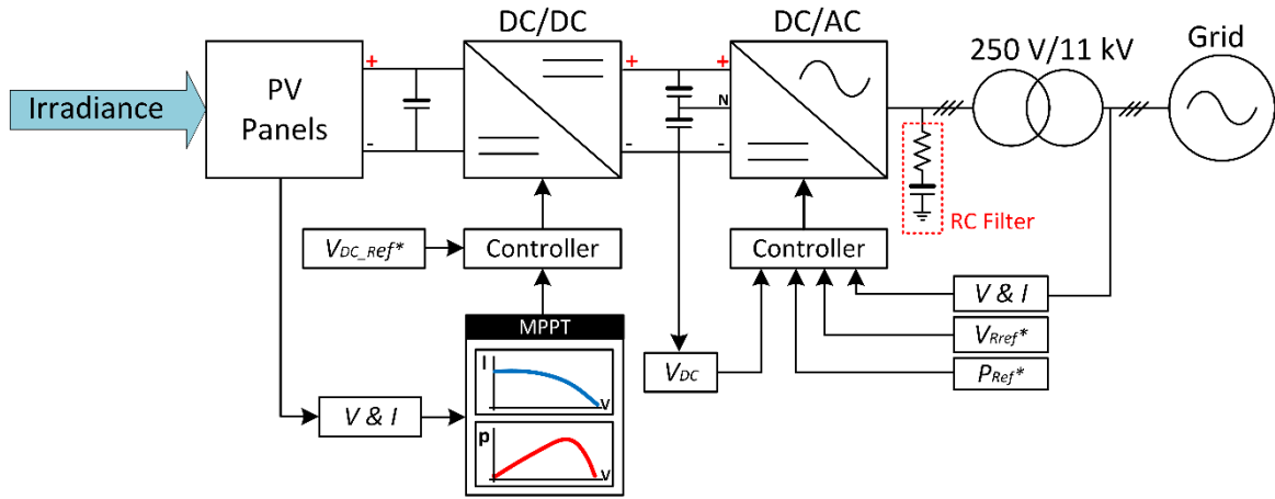
Figure 5. PV Model
