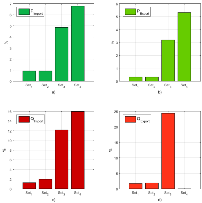
Figure 32. ROCOF NDZs for Generation Mix 4, a) Active power import, b) Active power export, c) Reactive power import, d) reactive power export
