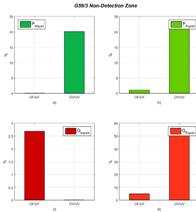
Figure 41. OF,UF,OV,UV NDZs for Generation Mix 8, a) Active power import, b) Active power export, c) Reactive power import, d) reactive power export
