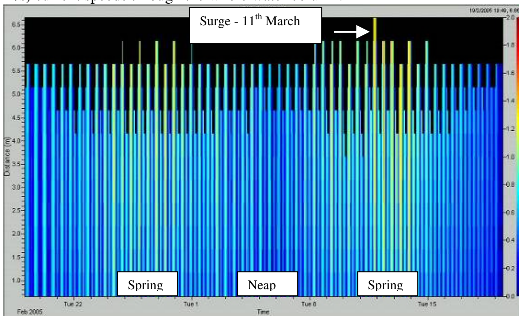
Figure 9 – Time-series of current speed profiles from the upward looking ADP on the Scroby Bank showing the spring - neap cycle and a wind-driven surge of 11 th -14th March 2005 at 20:00 GMT. Colour bar on right shows current speeds (m/s).
