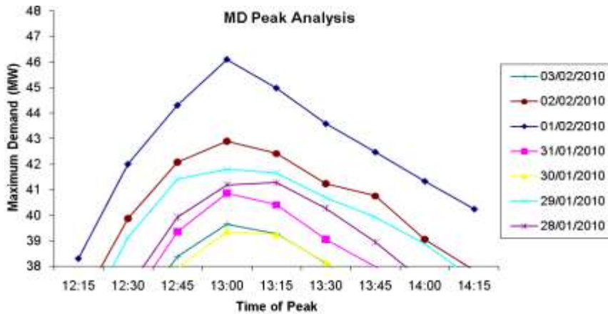
Figure 34 - Winter demand peak analysis
