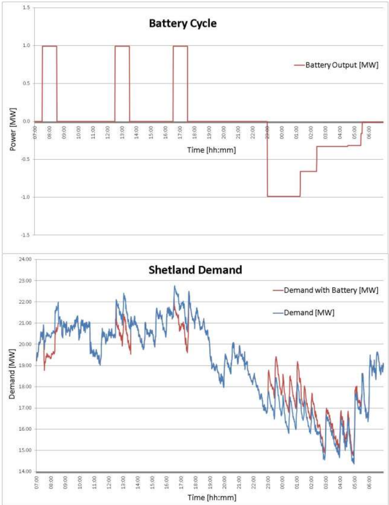
Figure 33 - Battery providing a reduction in peak demand
